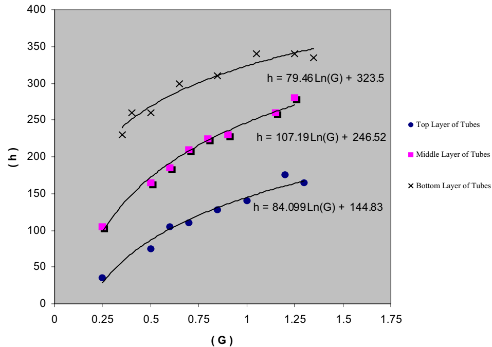
Fig ( 5 ) Heat Transfer Coefficients for Different Layers of Tube - Bundle
