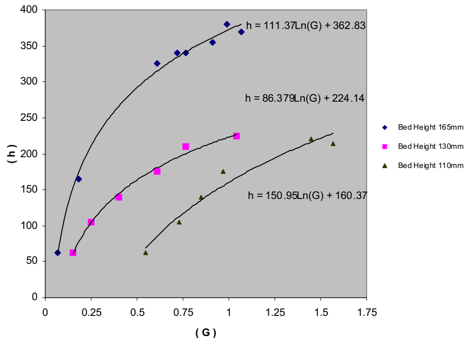
Fig (3) Relations between Heat Transfer Coefficient and Superficial Mass Velocity for Single Tube
