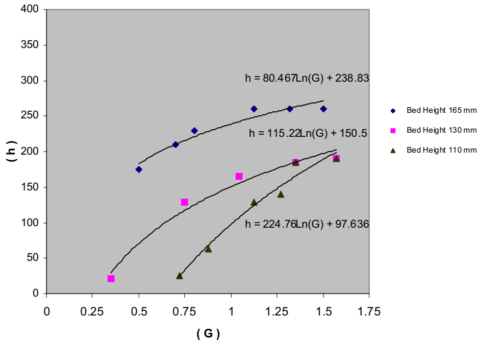
Fig (4) Relations between Heat Transfer Coefficient and Superficial Mass Velocity for Tube Bundle
