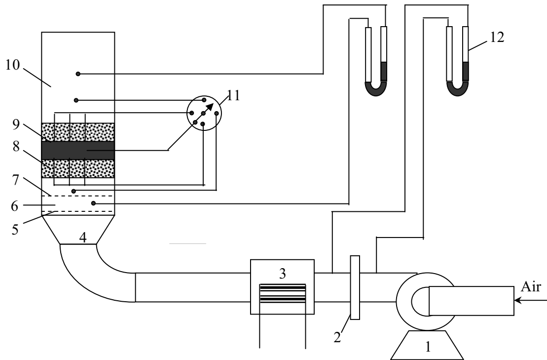
Fig (1) Scheme of Facilities
